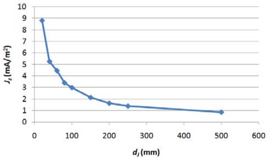
Figure 33: Current density J_z versus distance d_J for exposure directly under the E4 bulb.
