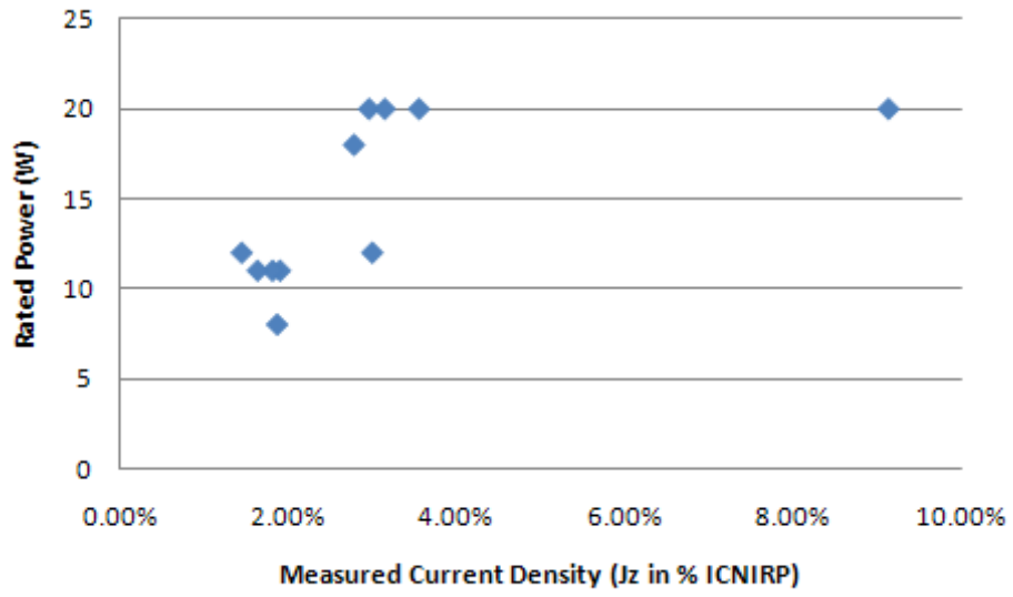
Figure 32: Current density J_z vs output power for the eleven ESBs investigated at a separation distance of 20 mm.
