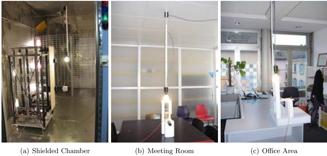
Figure 42: Bulb hanging from the ceiling is measured in different environments to test the dependance of surroundings on bulb measurements.
